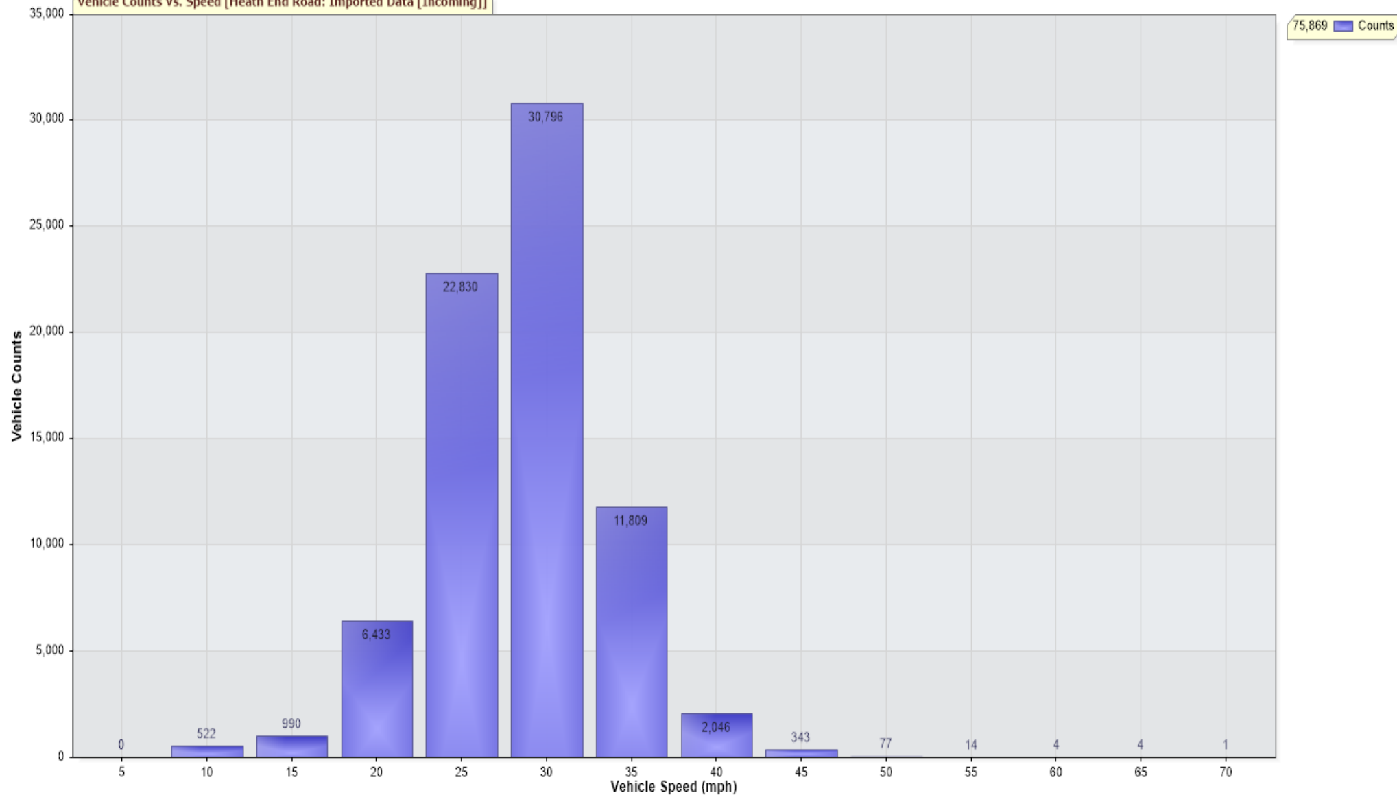
Vehicle Counts Vs. Speed [Heath End Road: Imported Data [Incoming]]
