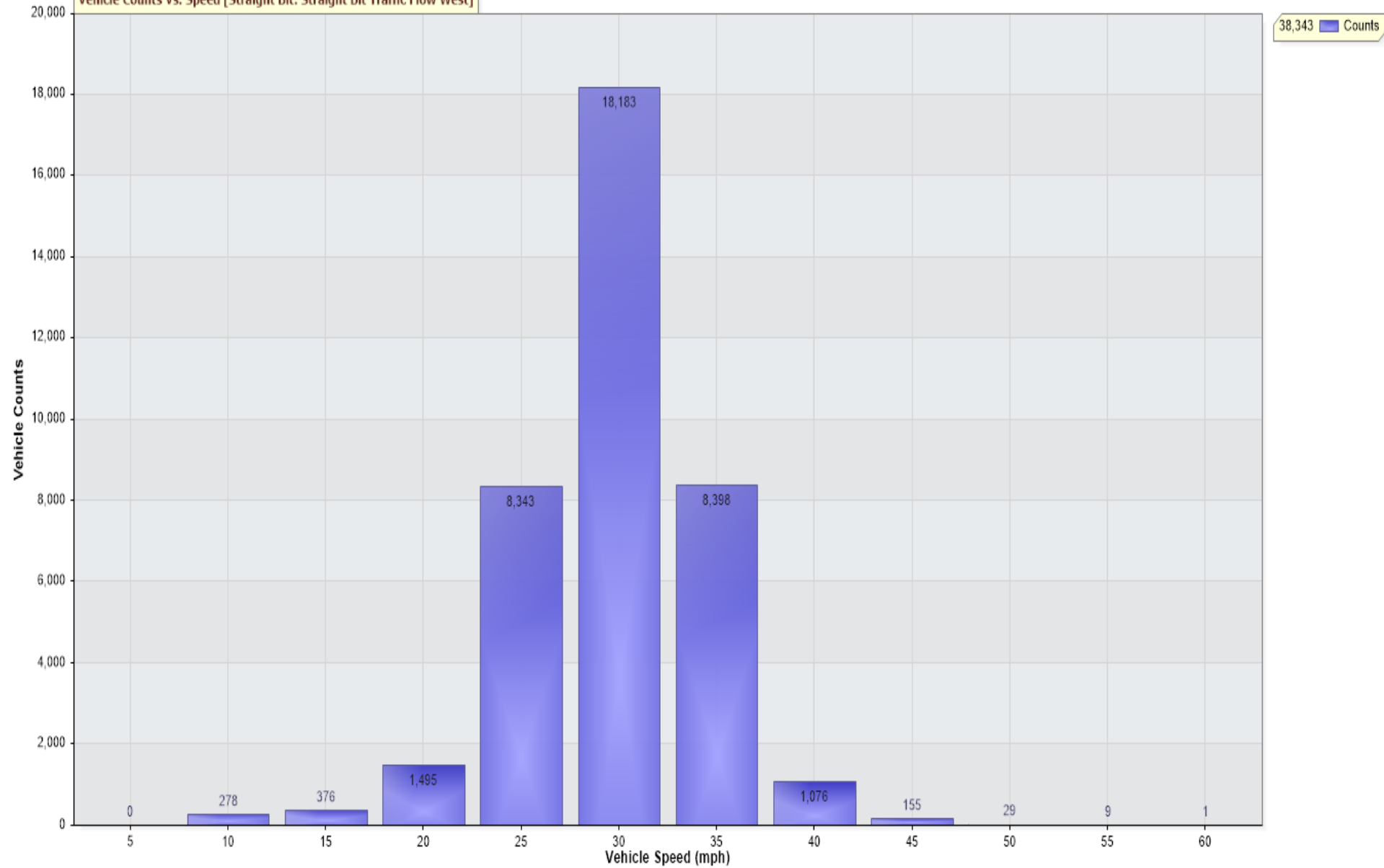
Vehicle Counts Vs. Speed [Straight Bit: Straight Bit Traffic Flow West]
