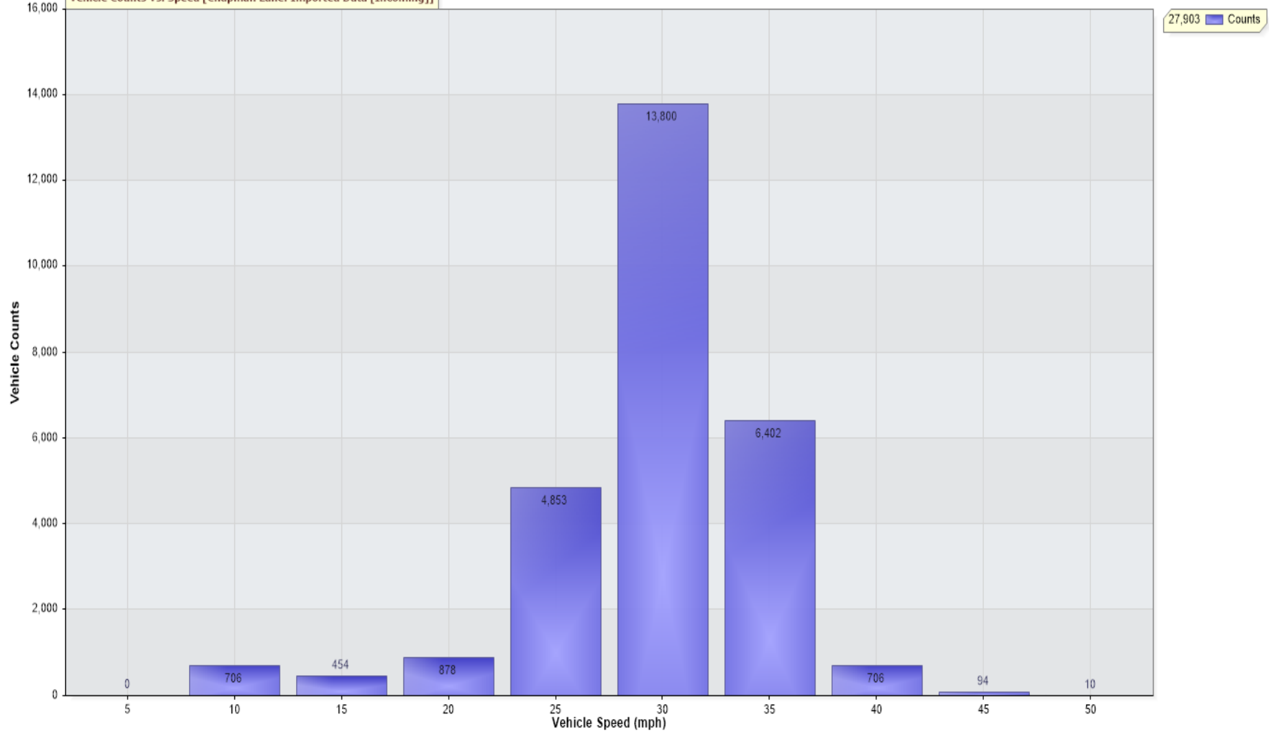
Vehicle Counts Vs. Speed [Chapman Lane: Imported Data [Incoming]]
