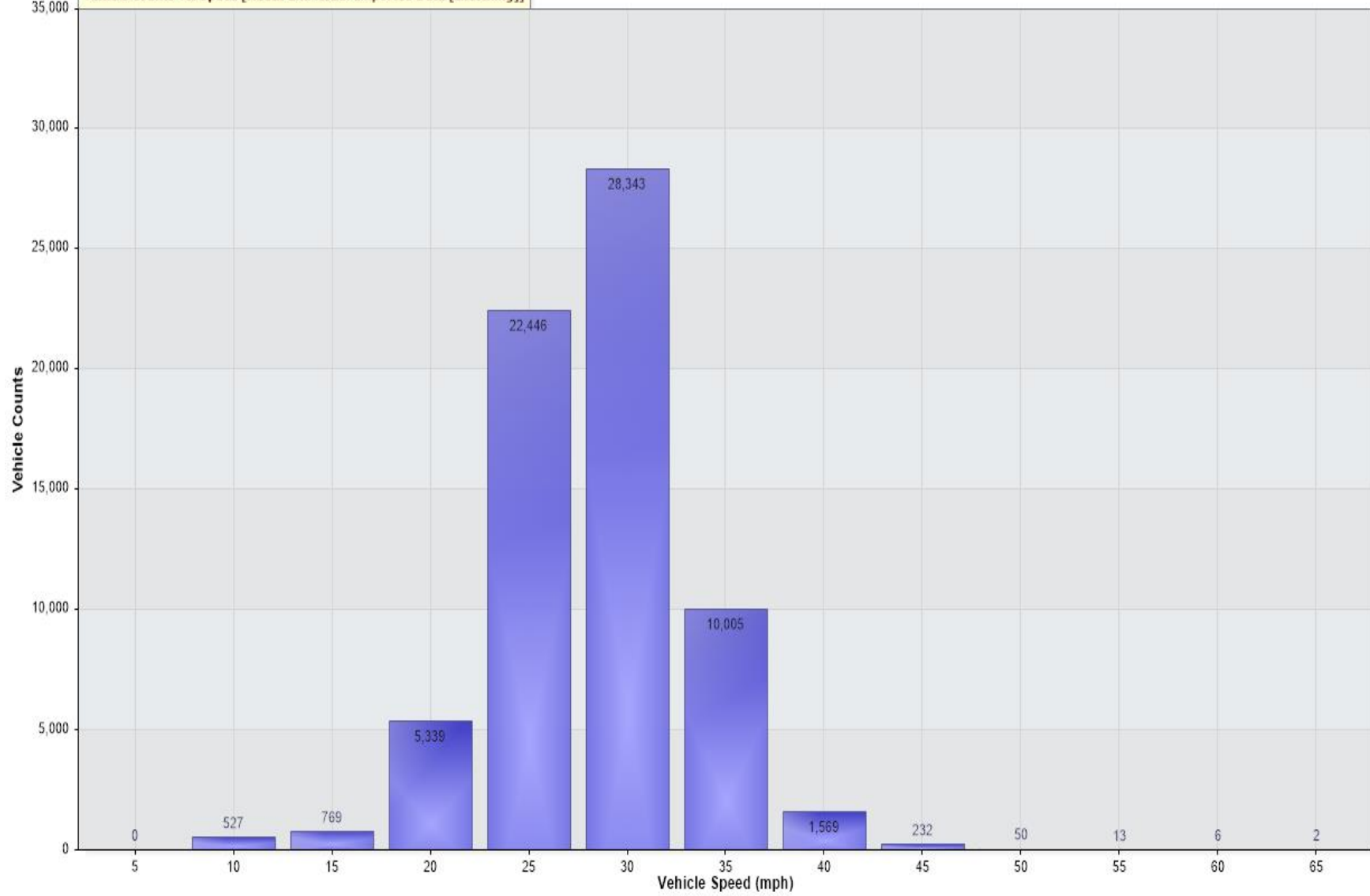
Vehicle Counts Vs. Speed [Heath End Road: Imported Data [Incoming]]
