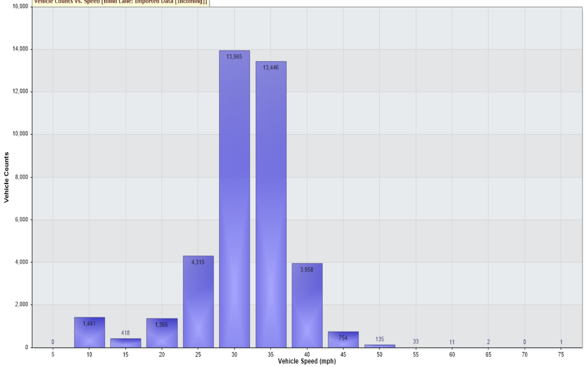
Vehicle Counts Vs. Speed [Blind Lane: Imported Data [Incoming]]
